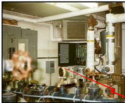
INSIDE NOATAK WATER TREATMENT PLANT
