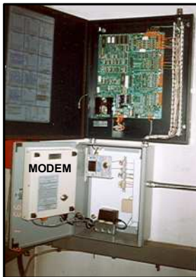
TYPICAL STAND ALONE DIRECT DIGITAL CONTROLLER (DDC) INSTALLED IN ALL REMOTE SITES
